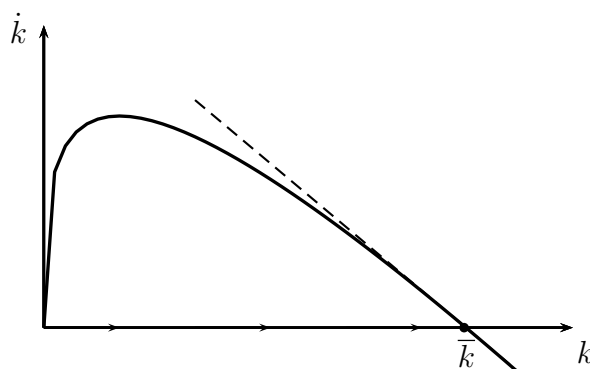
Figure 4.1: Phase diagram: exact and approximated
